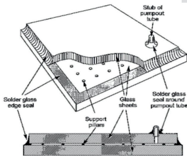
Figure 3. VIG - Operating diagram of one of the VIG on the market.
