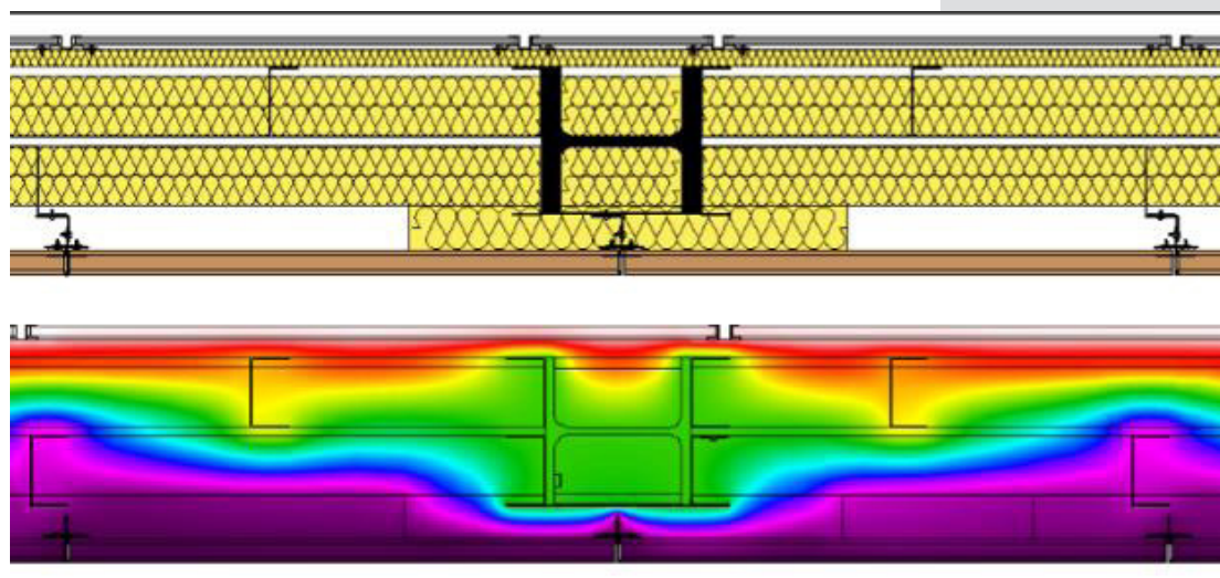
Figure 9. Thermal distributions diagram for the thermal bridges control.
