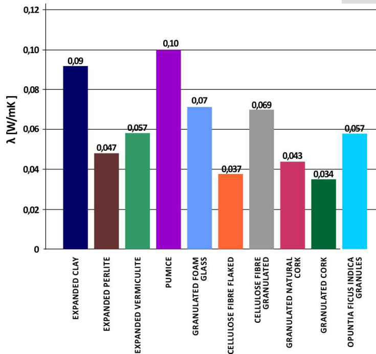
Figure 7. Comparison of thermal conductivity of bulk granules with commercial ones.
