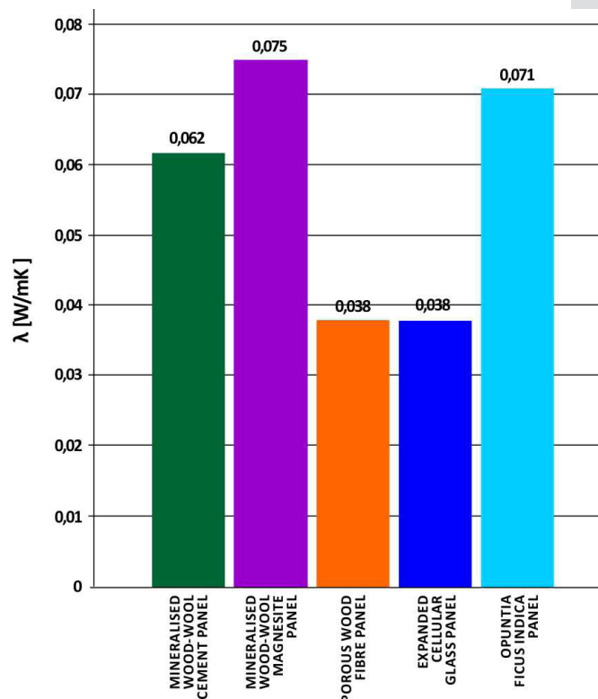
Figure 8. Comparison of thermal conductivity of panels with commercial ones.
