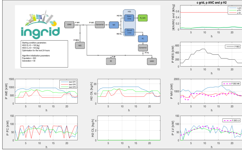
Figure 4. The Graphic User Interface (GUI) of the optimizer application developed in MATLAB® environment.
