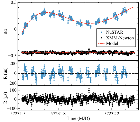
Figure 3. Top panel - Pulse phase delays as a function of time computed by epoch-folding 300 second data intervals of the XMM-Newton observations and 500 second data intervals of the NuSTAR observation. Red dotted line represents the best-fit model (see text for more details). Middle panel - Residuals in \mu\text{s} of the NuSTAR data with respect to the best-fitting orbital solution. Bottom panel - Residuals in \mu\text{s} of the XMM-Newton data with respect to the best-fitting orbital solution.
