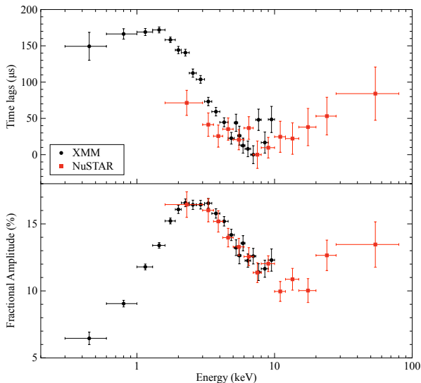
Figure 4. Top panel - Time lags in \mu\text{s} evolution as a function of energy obtained from the XMM-Newton and NuSTAR observations reported with black dots and red squares, respectively. For display purpose only the reference pulse profiles of the two datasets has been set around 7 keV. Bottom panel - Evolution of the pulse fractional amplitude for the two datasets. The colour coding has been kept fixed between the panels.
