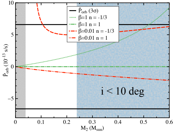
Figure 7. Orbital period derivative versus companion star mass in the hypothesis of conservative and non-conservative mass transfer (with mass leaving the system with the specific angular momentum at the inner Lagrangian point). Dotted and dashed-dotted green curves represent the conservative ( \beta = 1 ) mass-transfer scenario assuming a low-main sequence ( n = 1 ) and a fully convective ( n = -1/3 ) companion star, respectively. Dashed and dot-dot-dashed red curves represent the non-conservative ( \beta = t_{out}/t_{quiet} \simeq 0.01 ) mass-transfer scenario again for a low-main sequence ( n = 1 ) and a fully convective ( n = -1/3 ) companion star, respectively. The horizontal black lines delimit the 3\sigma orbital period derivative confidence level interval obtained from the analysis. Finally, vertical lines represent the minimum mass estimated from the binary mass function (for a 1.4 M_{\odot} NS) and the companion mass for an almost face-on system ( i=10^{\circ} ).
