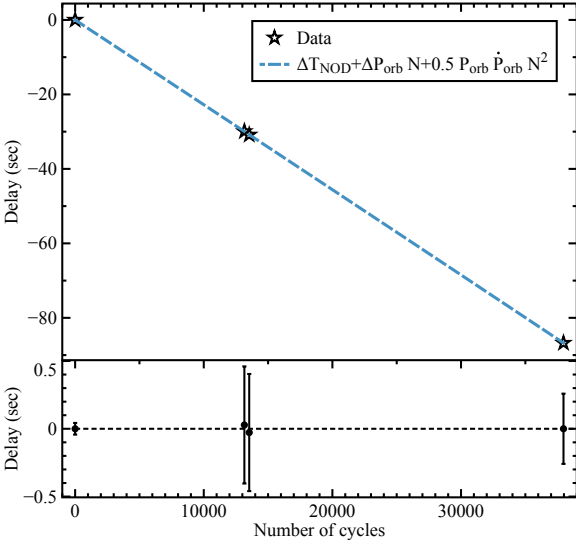
Figure 6. Top panel - Time delays of the NS time of passage from the ascending node for each of the observed outbursts of IGR J00291+5934. The cyan dashed line represents the best-fitting parabola used to model the data. Bottom panel - Residuals in seconds of the time delays with respect to the best-fitting timing solution.
