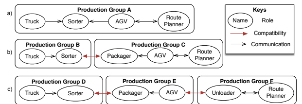
Figure 1: Social design choices for production groups.
