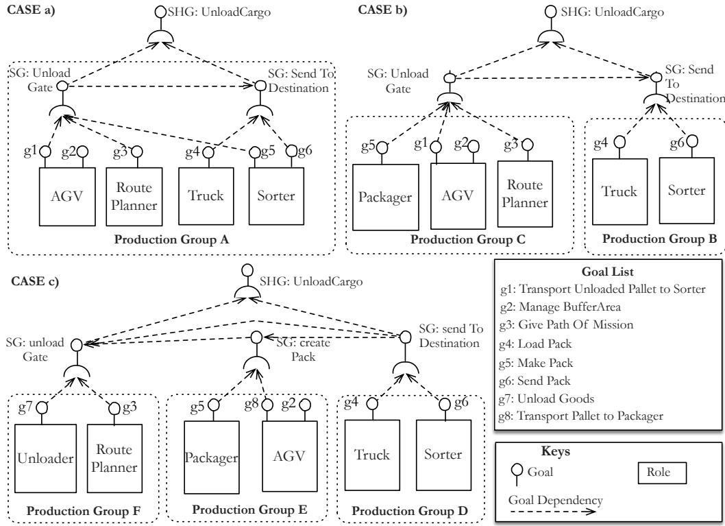
Figure 2: Different functional design choices for Production of a super-holon.
