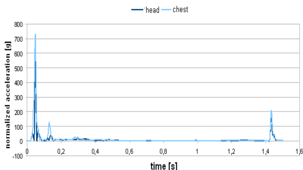
Figure 3: Head and chest acceleration in the side impact with Pick Up at 40km/h
