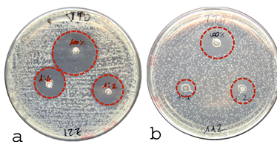
Fig. 1. Agar well diffusion method. Different inhibition halo diameters (red circles) for Tea tree Oil (concentrations 100%, 50%, 25%) referred to Bacillus subtilis (a) and Micrococcus luteus (b).
